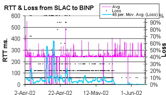
Figure 5: Effects of network upgrades made to the BINP network in May of 2002. The thick light shaded line is to guide the eye and is the rolling average loss for the previous 24 hours
