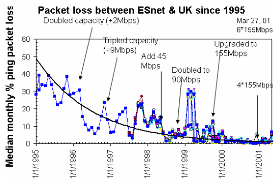
Figure 4: Network performance between ESnet Monitoring-hosts in the U.S. and Remote-hosts in the U.K
